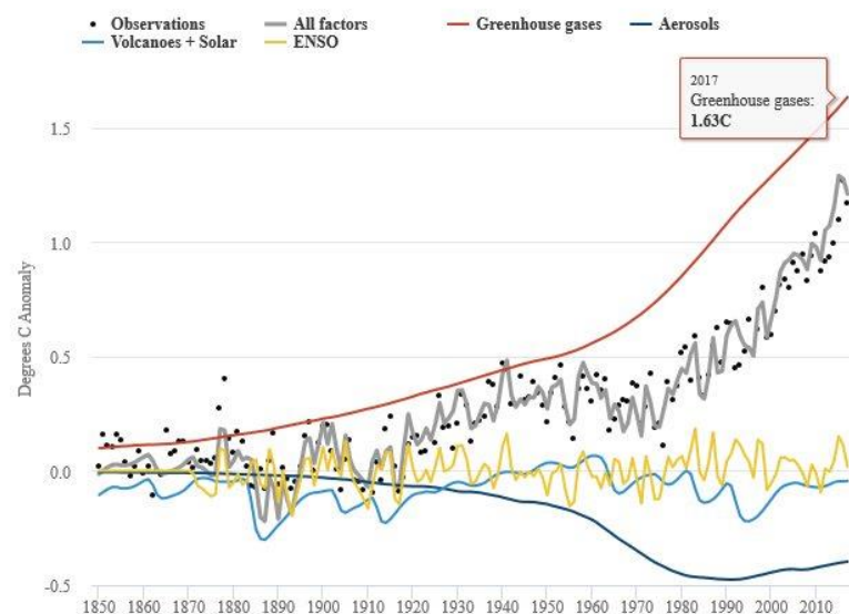
Components of temperature change
